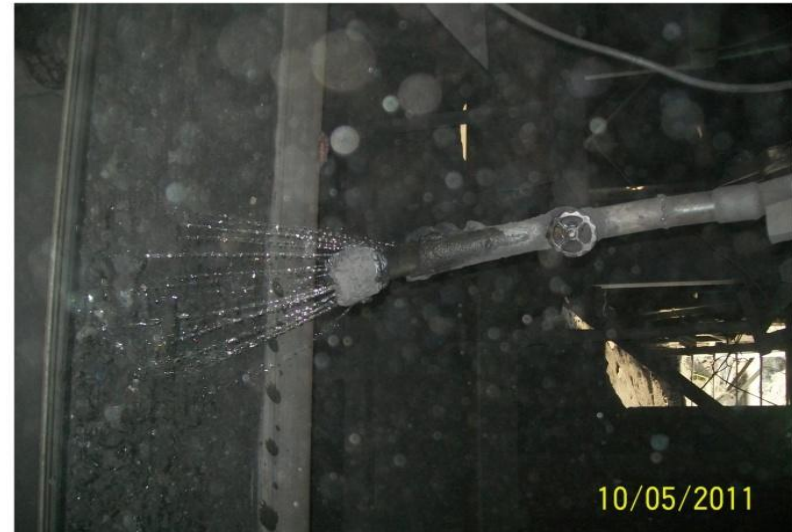
Dust Suppression System in Coal Handling Plant at PTPS
